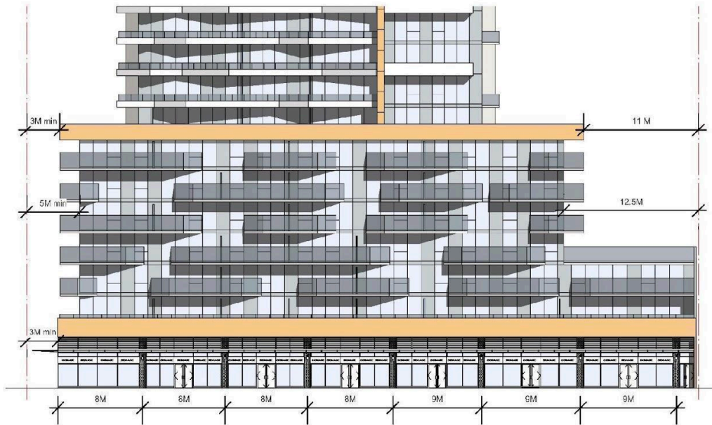
SOUTH ELEVATION
