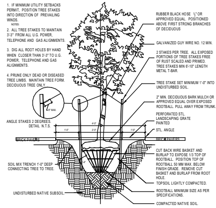
typ. tree planting detail
