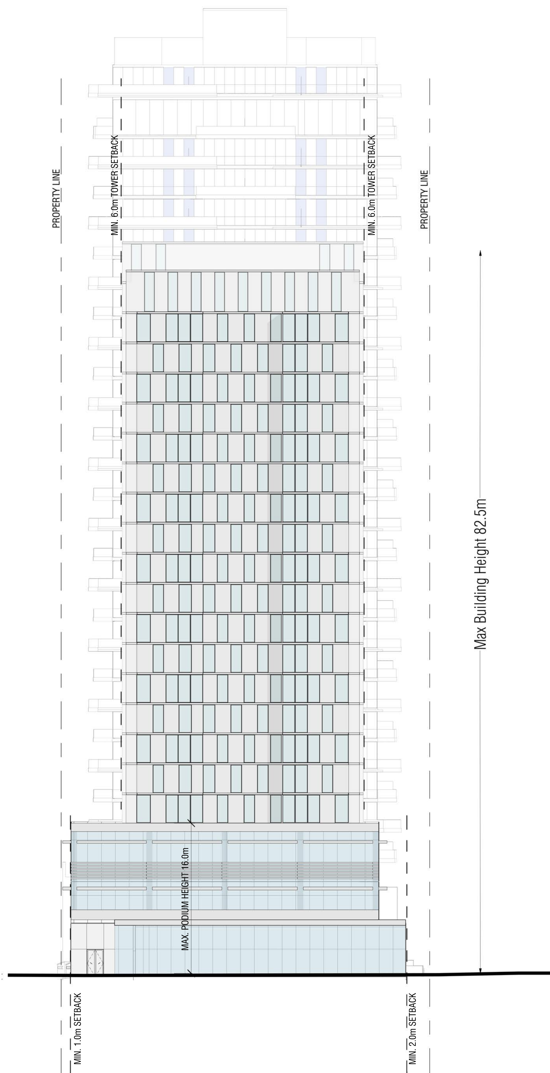
WEST ELEVATION
