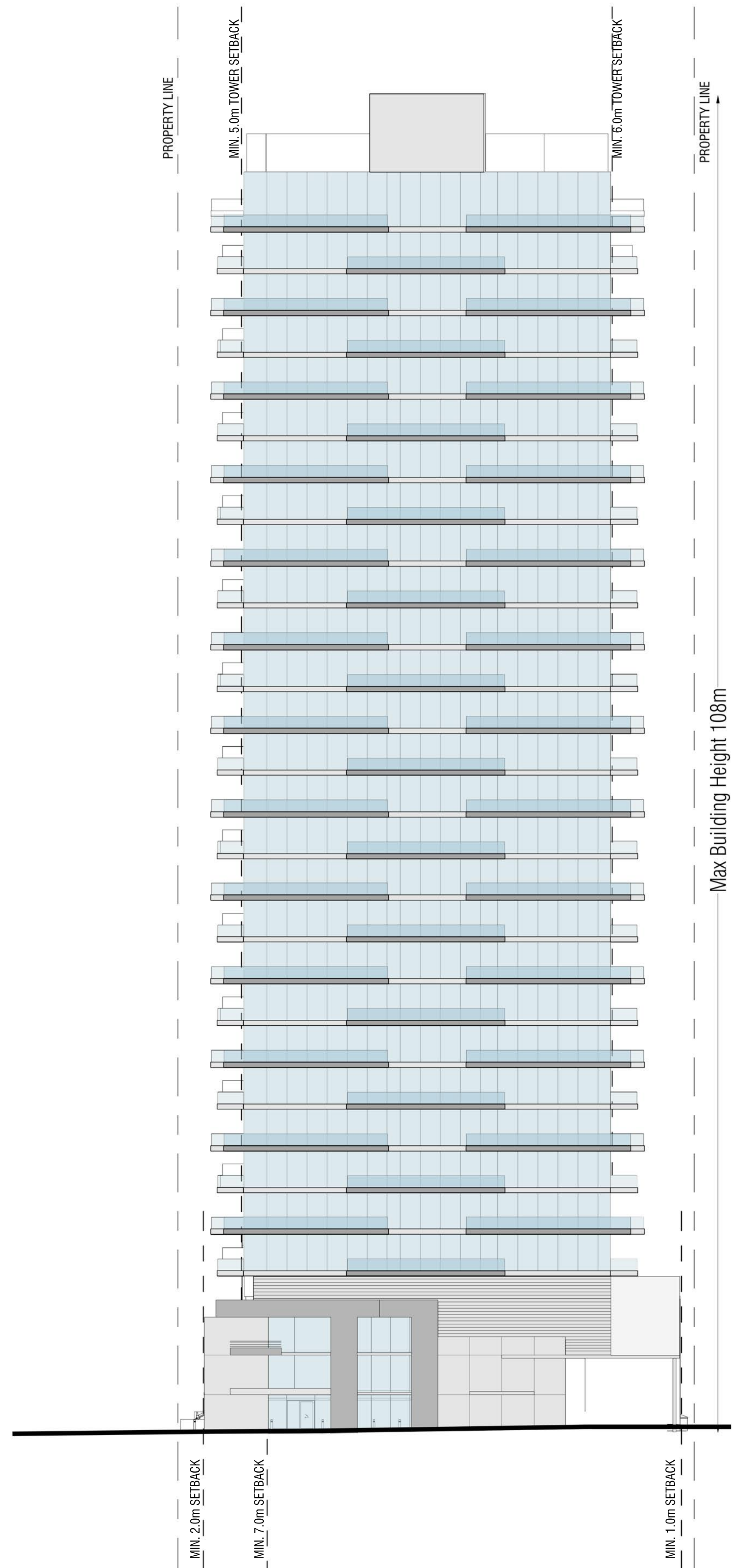
EAST ELEVATION
