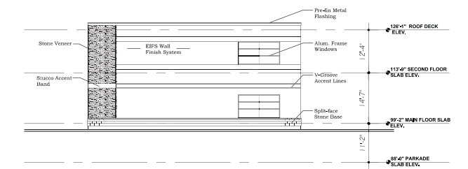
4 South Elevation 1" = 25'-0"
