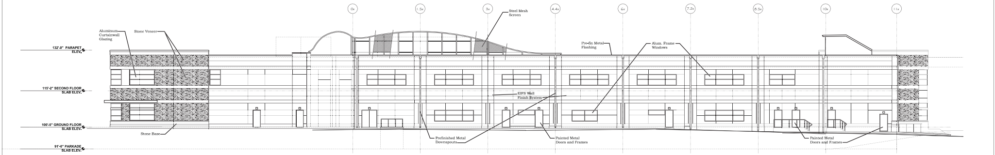
2 North Elevation 1" = 25'-0"
