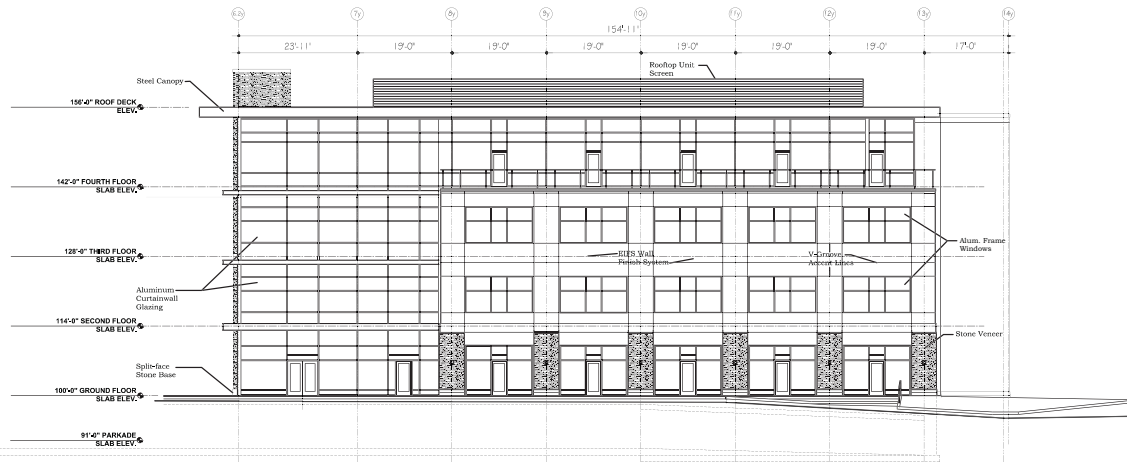
1 East Elevation 1" = 25'-0"
