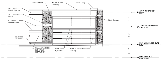
2 South Elevation 1" = 25'-0"
