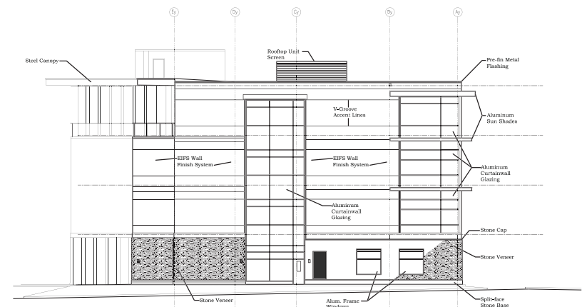
4 North Elevation 1" = 25'-0"
