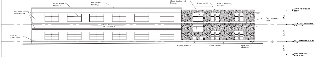
3 West Elevation 1" = 25'-0"
