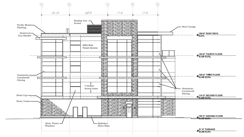
2 South Elevation 1" = 25'-0"
