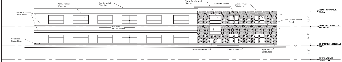
3 West Elevation 1" = 25'
