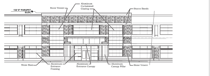
4 Main Entrance Elevation 1" = 25'-0"
