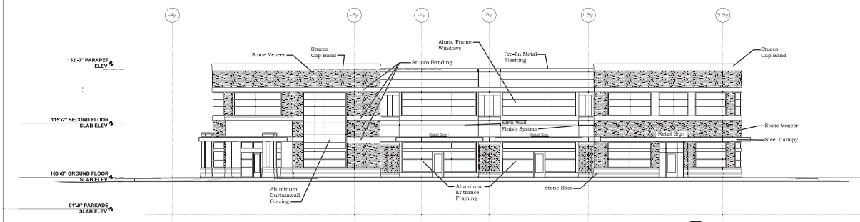
3 East Elevation 1" = 25'-0"
