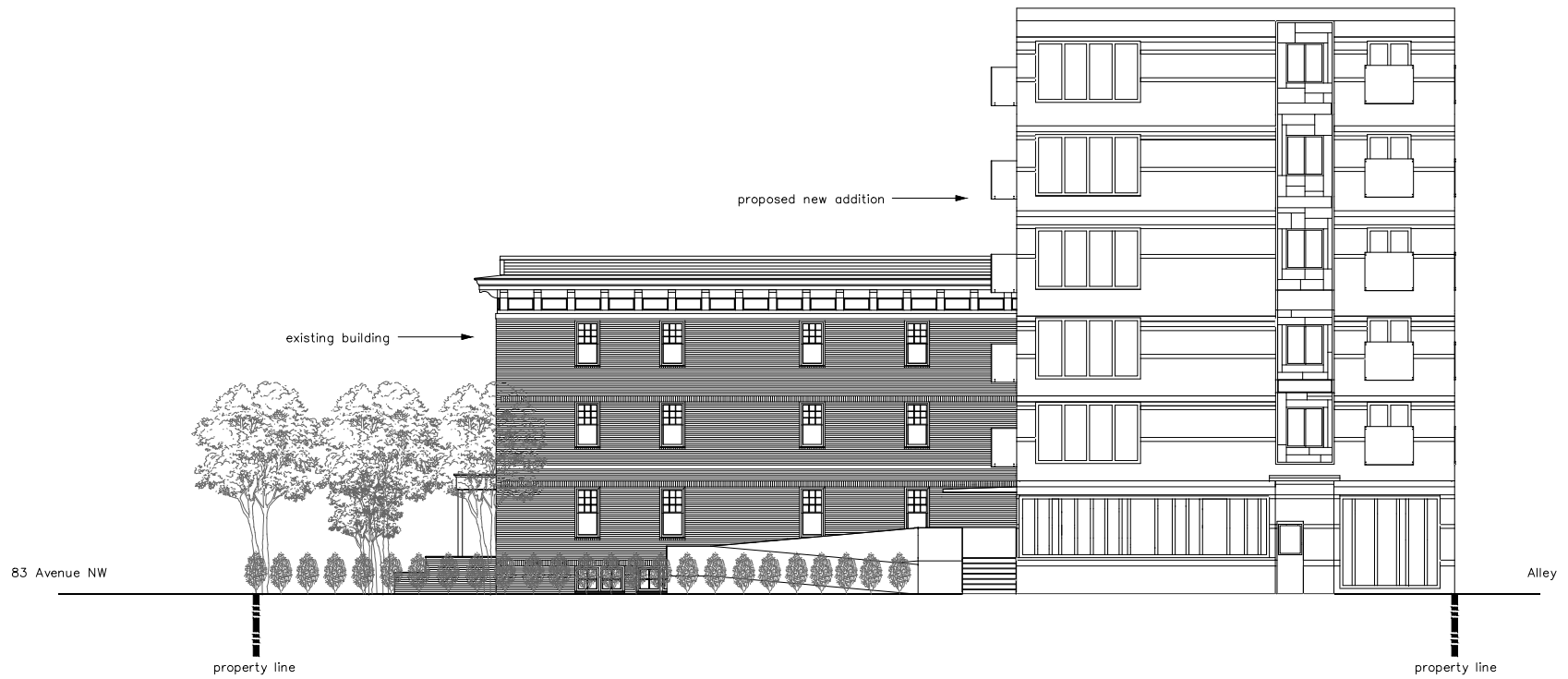
Elevation – West
