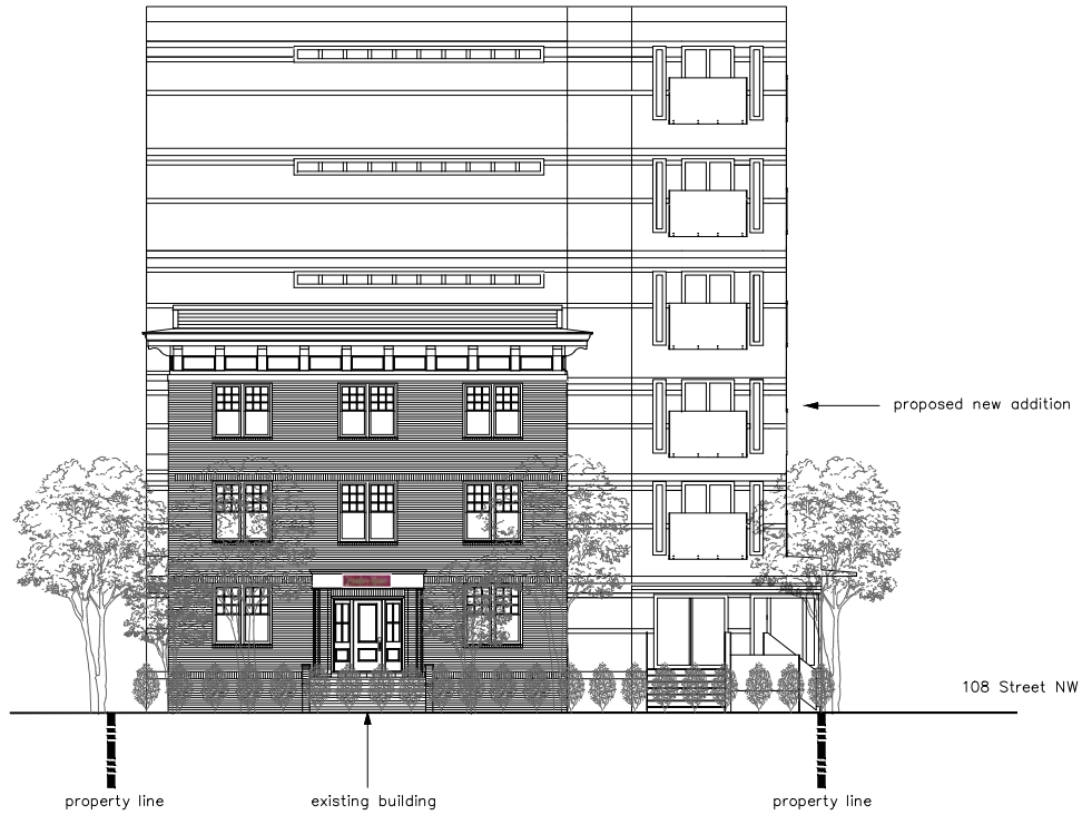
Elevation – North
