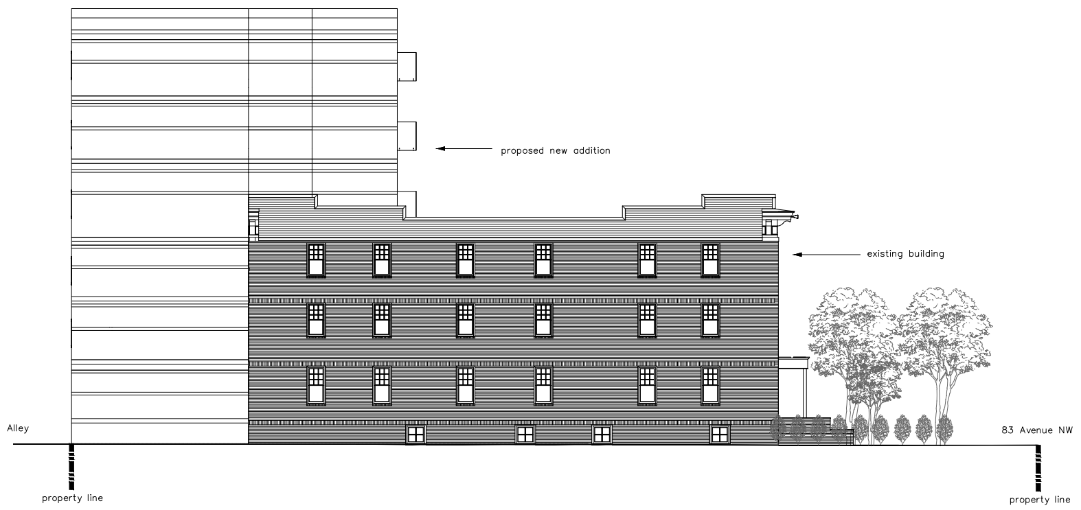
Elevation – East
