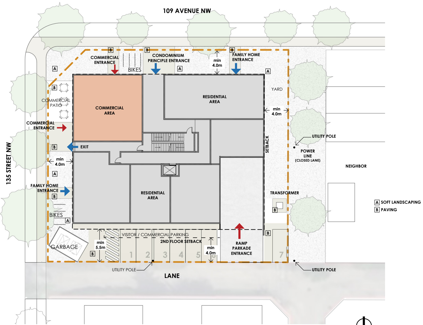
SITE PLAN
