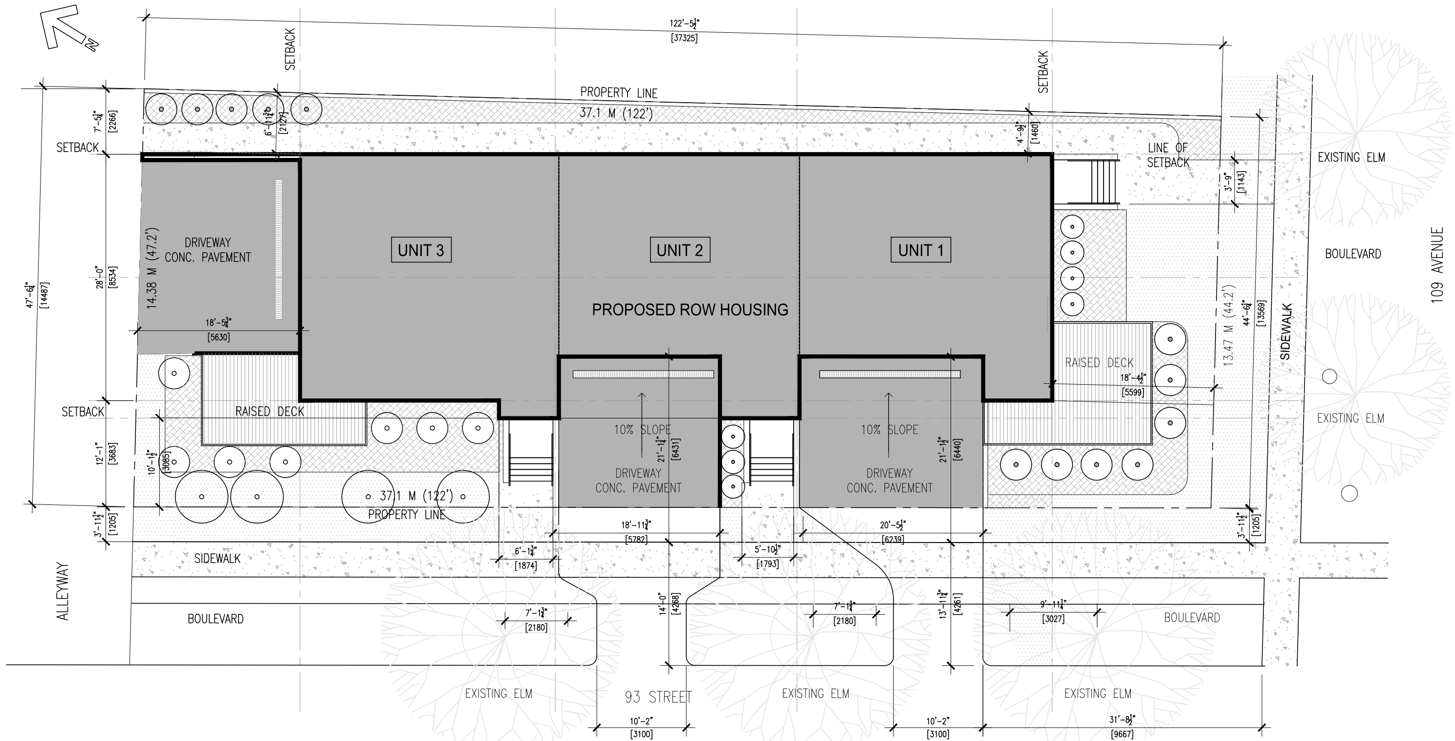
1 SITE DEVELOPMENT PLAN A1.1 SCALE: 3/32"=1'-0"
