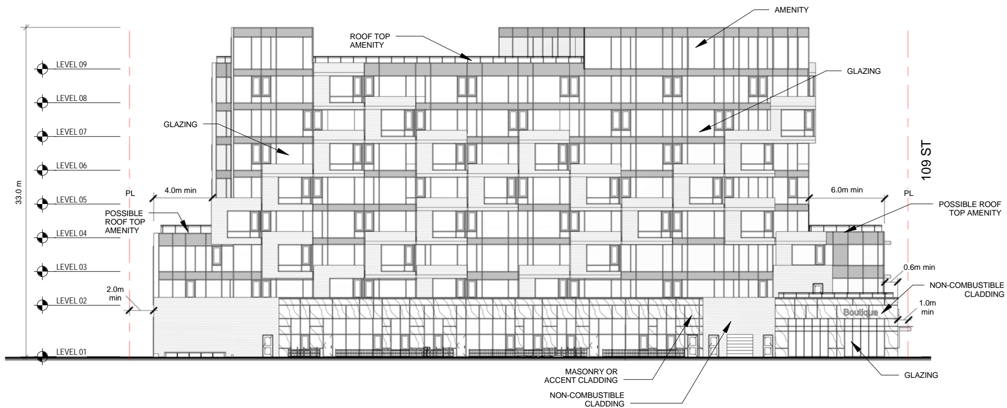
NORTH ELEVATION - ALONG LANE
